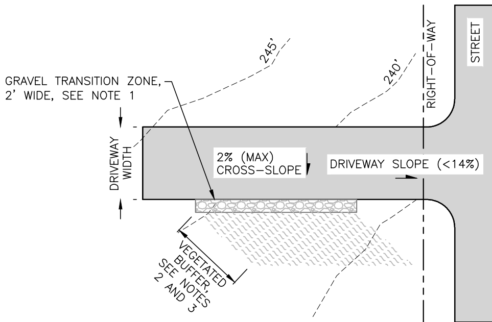
PLAN — FLAT DRIVEWAY (≤5%)
